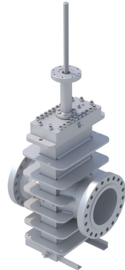
The fabricated API 6D gate valve in the GROVE valve portfolio helps to minimize product contamination in critical pipeline transmission and storage applications.
